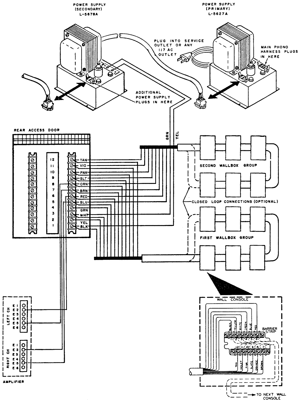
Electrical Connections
